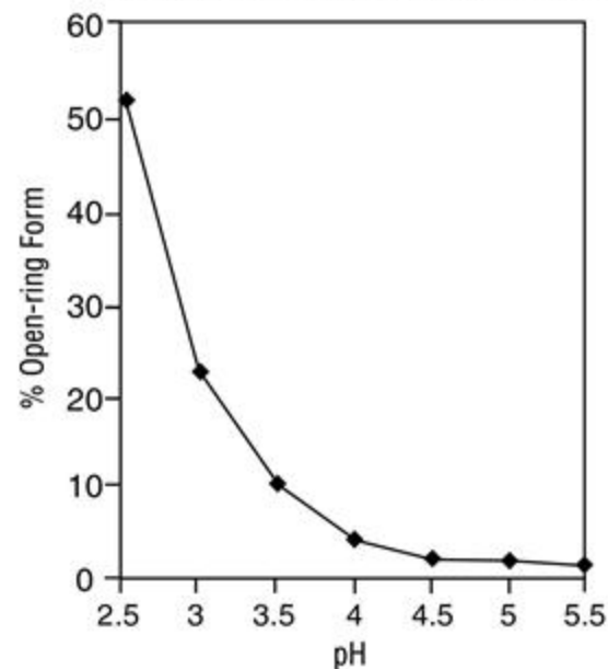
pH Dependence of Open-ring Form in Water
